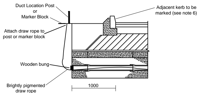
Detail at end of duct under carriageway
