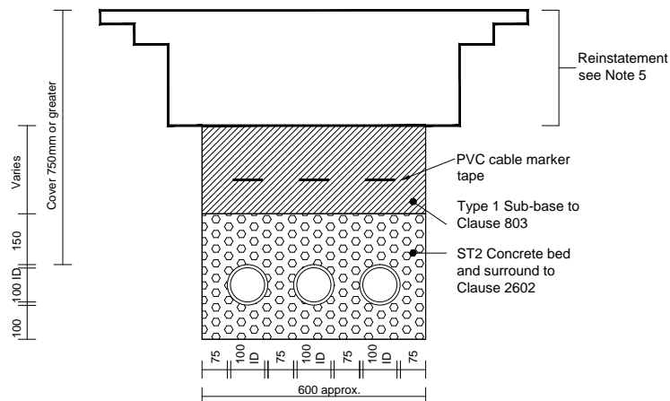
Carriageway with depth of cover exceeding 750 and 3 No. ducts
