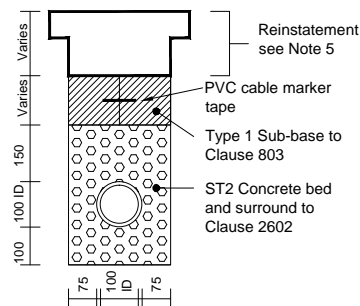
Footway with depth of cover 450 or greater
