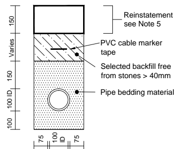
Verge with depth of cover 450 or greater
