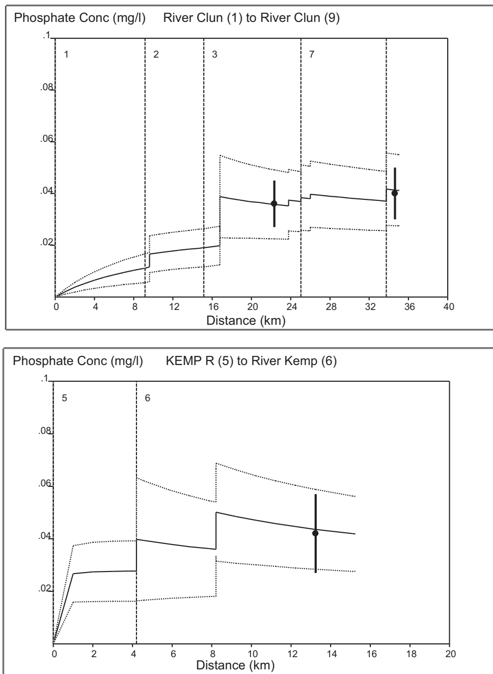
Figure K5: Modelled and observed \text{PO}_4 concentrations along the River Clun (top graph) and the River Kemp (bottom graph) after calibration. The solid black line indicates the modelled concentration with the dashed lines indicating the confidence limits. The black dot and lines indicate the observed mean (dot) concentration and confidence limits (lines).
