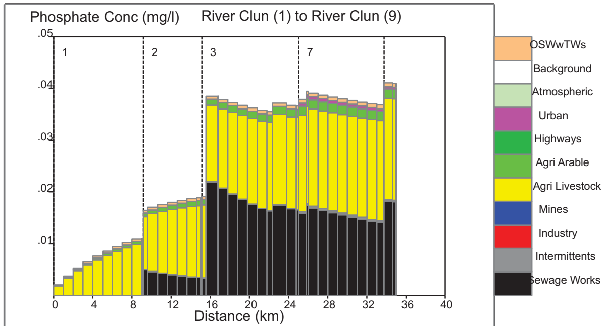
Figure K6: Downstream source apportionment of \text{PO}_4 concentrations along the River Clun after calibration.
