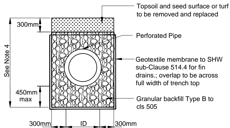
Typical Section through soakaway.
