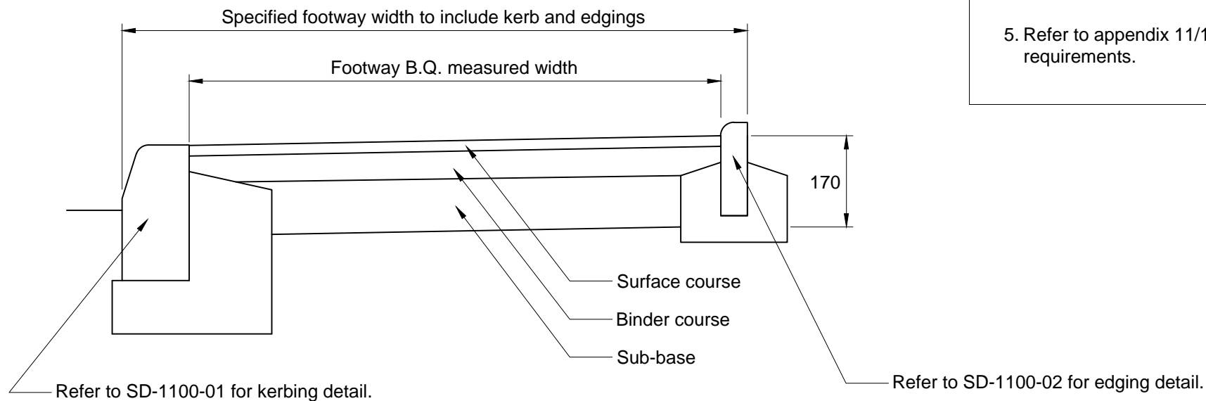
Typical Footway Type 1 Cross Section
