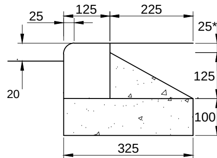
Type BN-125x150 Bullnose
