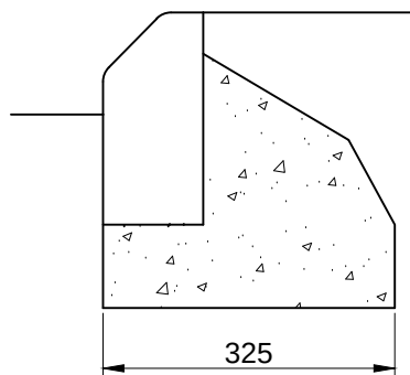
Type SP-125x255 45° Splay
