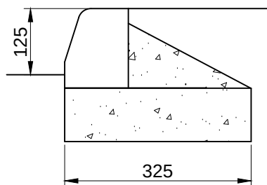
Type HB3-125x150 Half Batter
