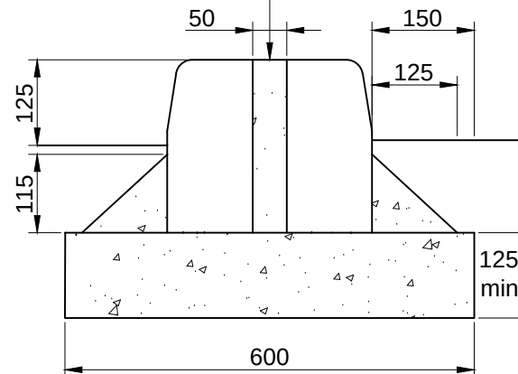
Type HB2D-125x255 Half Batter Double Kerbs
