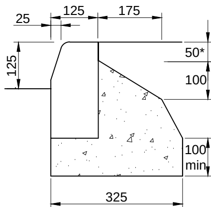
Type HB2-125x255 Half Batter
