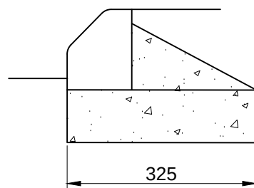
Type SP2-125x150 45° Splay (No longer a BSEN1340 product)
