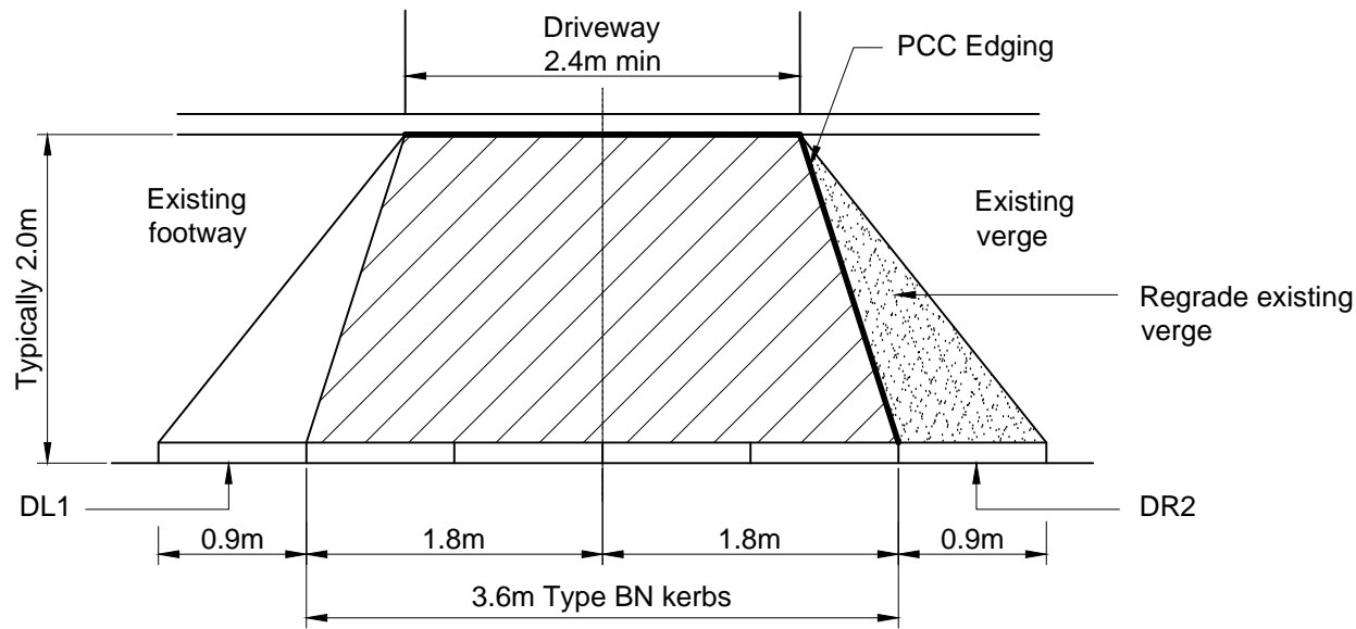
Typical Vehicular Crossing Plan View
