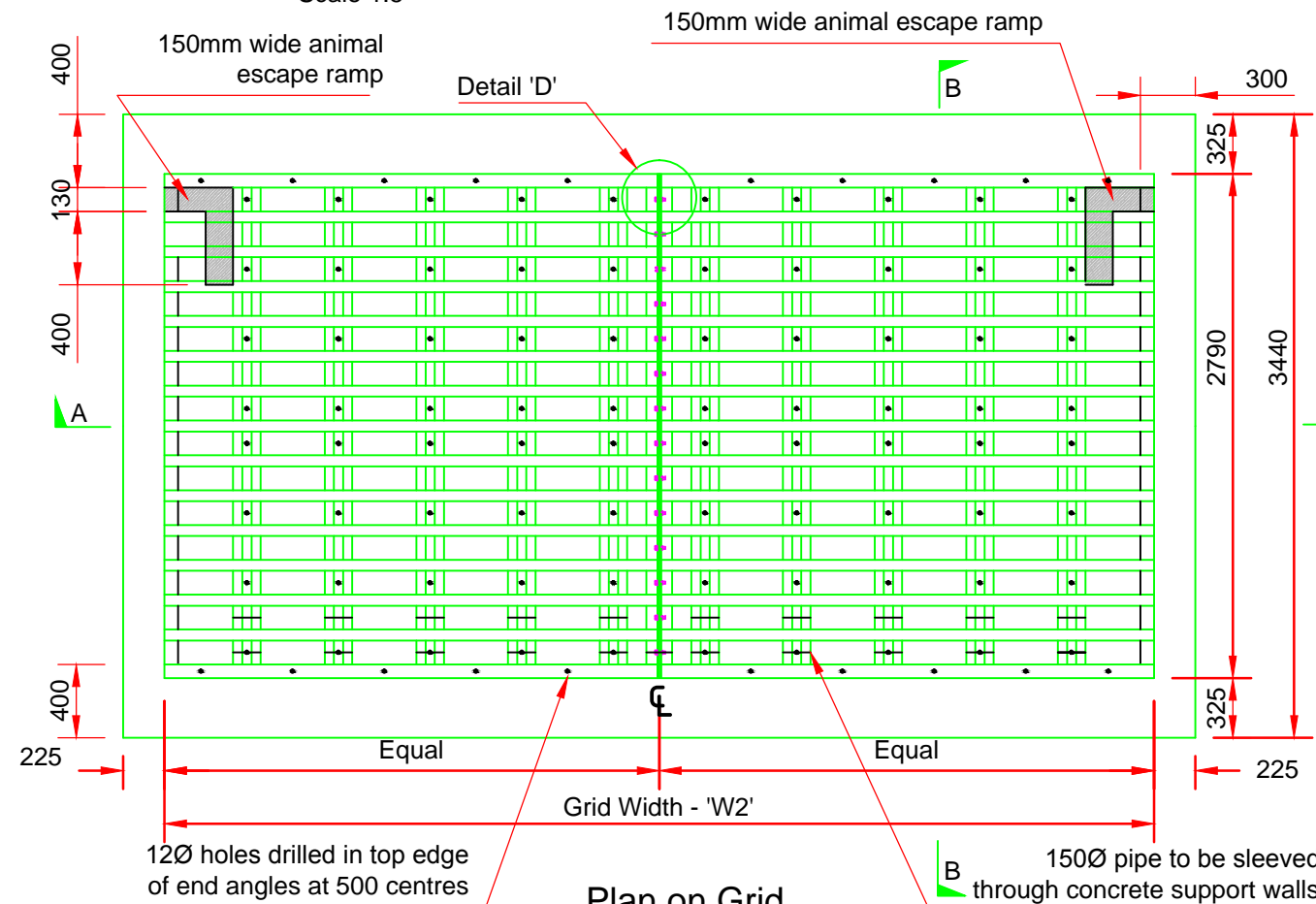
Plan on Grid Scale 1:40
