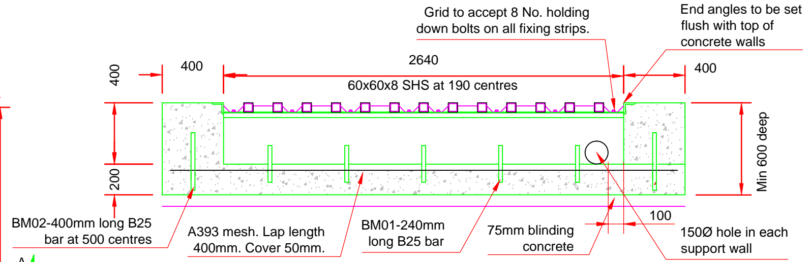
Section B-B Scale 1:25
