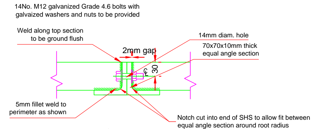
Section E-E Scale 1:5
