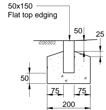
Edging Type EF
