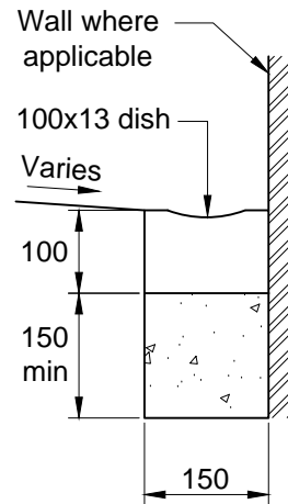
Channel Type CD2-150x125 dished (No longer a BSEN 1340 Product)
