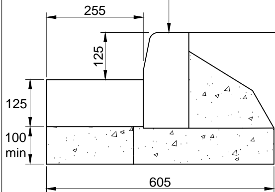
Channel Type CS1-255x125
