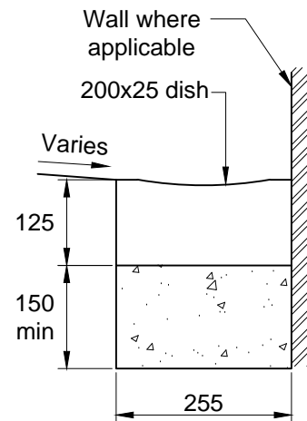
Channel Type CD-255x125 dished (Use where there are no DDA issues)
