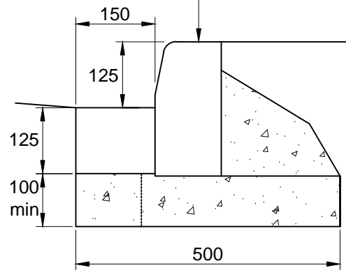
Channel Type CS2-150x125
