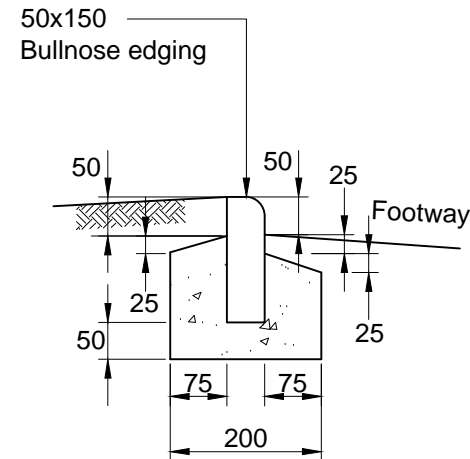
Edging Type EBN-Raised
