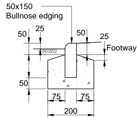
Edging Type EBN-Flush
